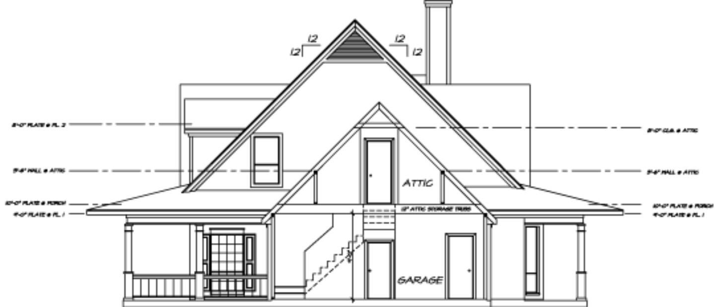
SECTION D-D BC 1/4" = 1'-0"
